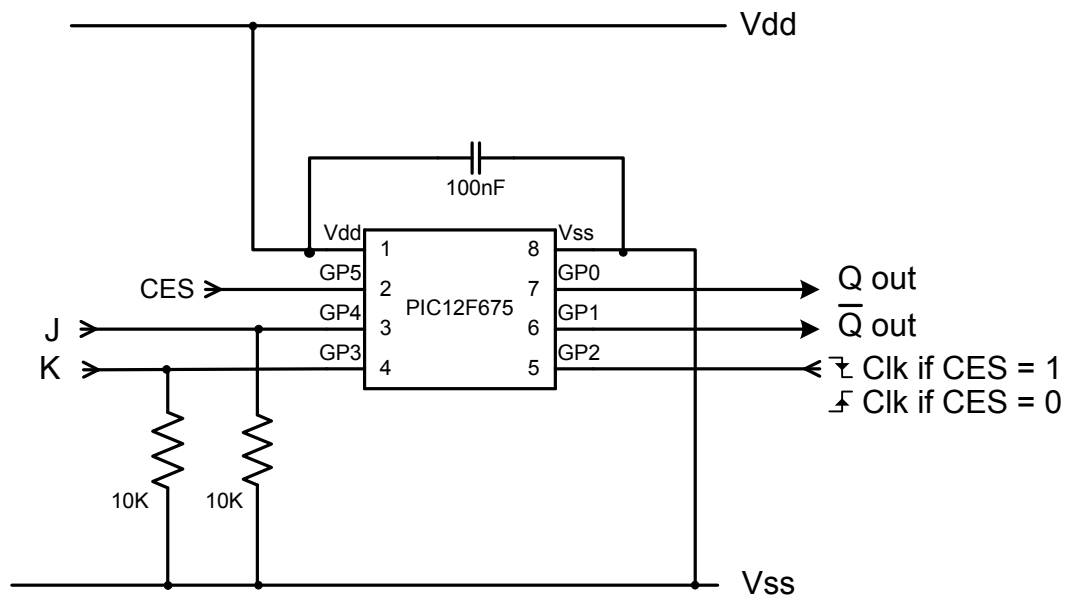
JK Type Flip Flop with selectable edge trigger clock
